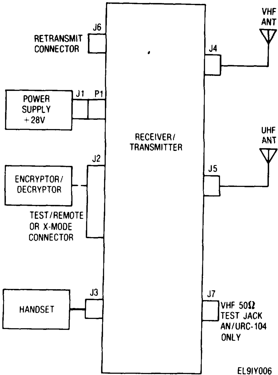
Figure 1-3. Radio Set Interconnect Diagram
